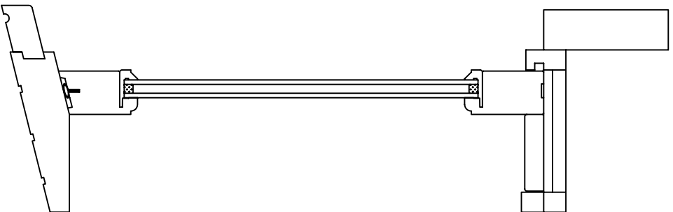
Vertical Cross Section
