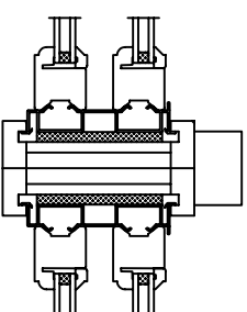
Mullion Detail
